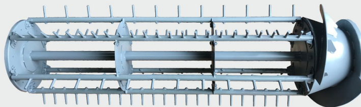
THRESHER DRUM WITH FEED AUGER (TRACK COMBINE)
